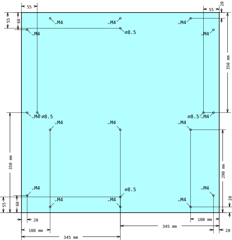
DRAWING 7, Pos 20 Hole placement
