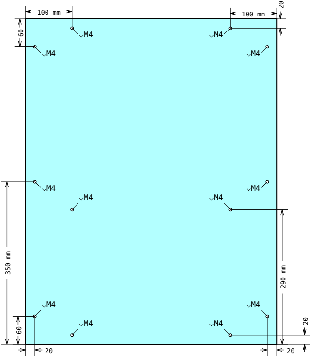
DRAWING 8, Pos 21 Hole placement
