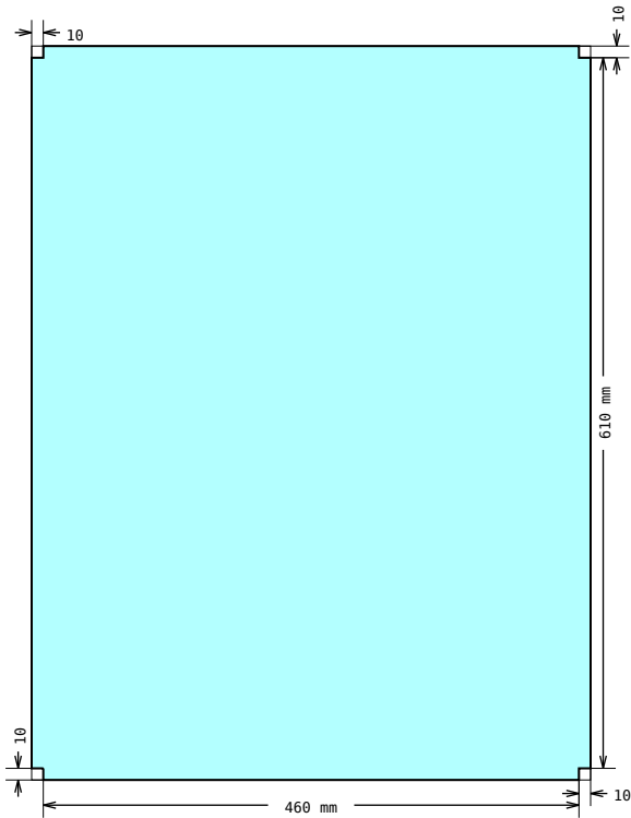
DRAWING 5, Pos 18 Shape measurements
