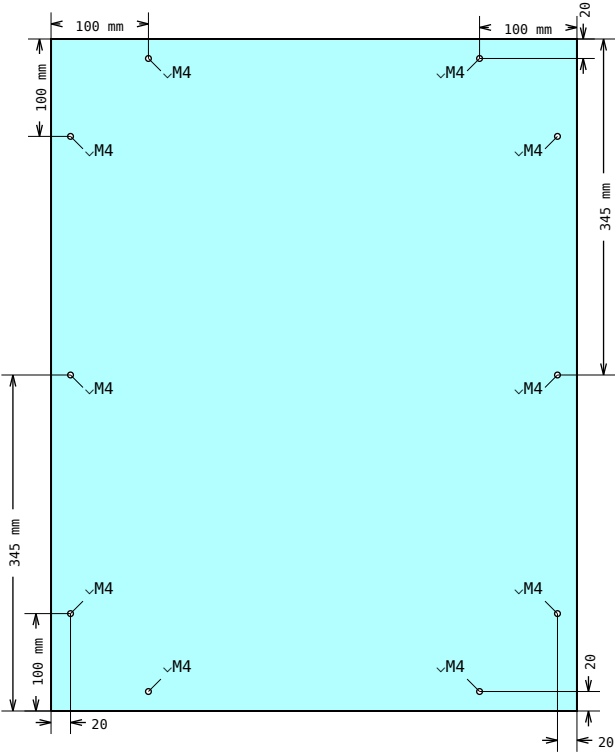
DRAWING 6, Pos 19 Hole placement
